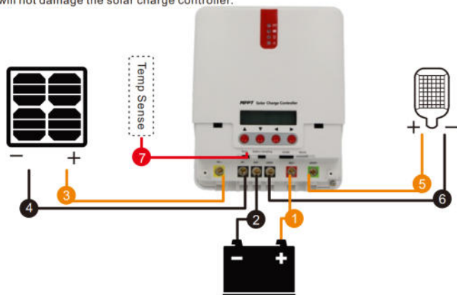
Figure 2-3 Wiring
