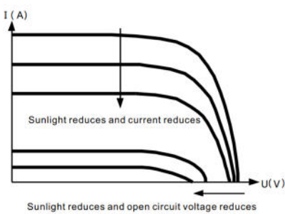
Figure 1-3 Solar Panel Output Characteristic and Lighting Relation
